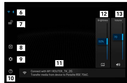
Fig. 2: Menu principal
